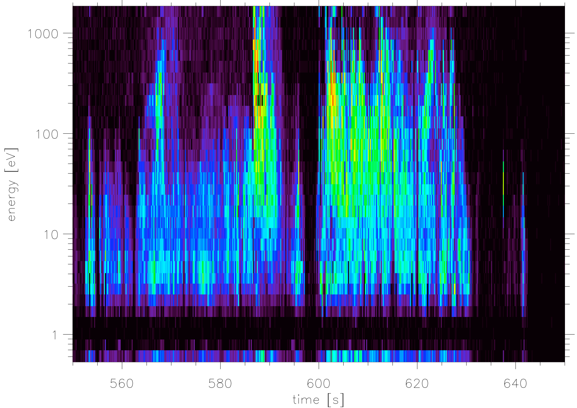
casc2 bg [differential energy flux]
