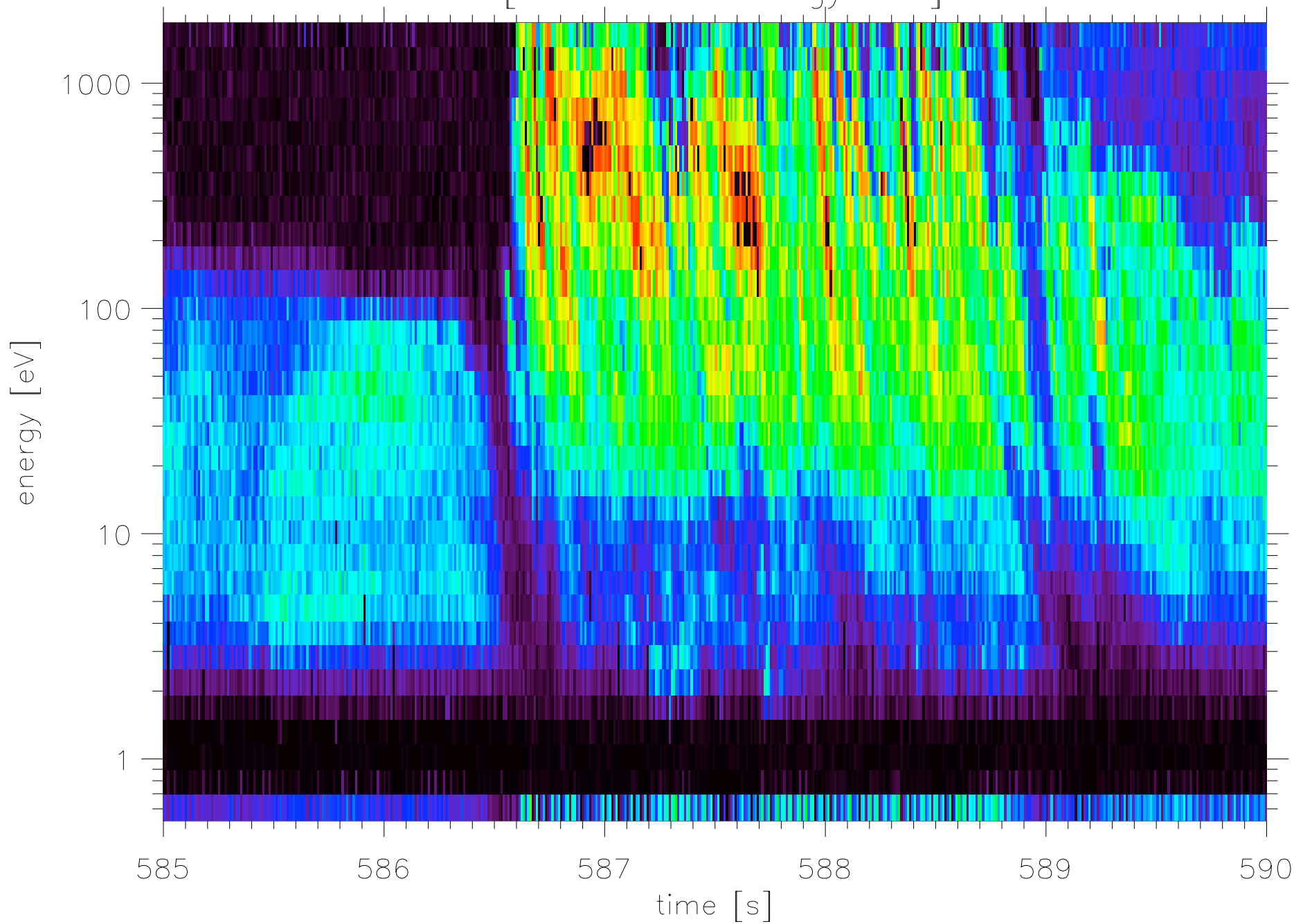
cas2 bg [differential energy flux]
