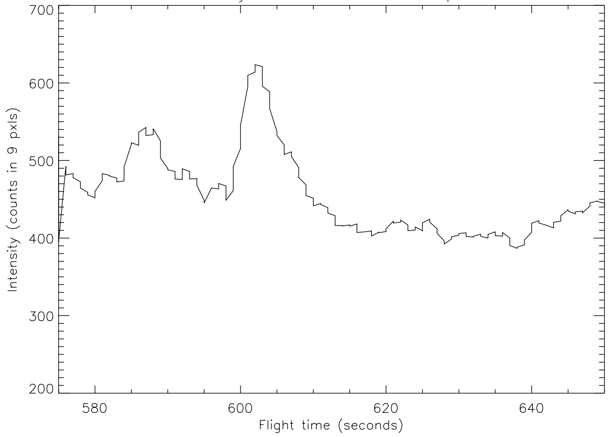
Intensity at rocket 150km-footprint
